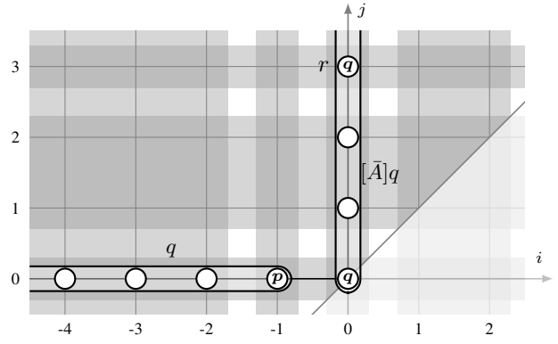
Figure 3: Canonical interpretation from Example 5.
