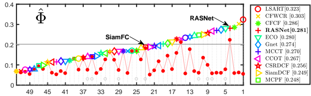
Figure 10. An illustration of the expected average overlap plot on the VOT2017 challenge. The gray horizontal line indicates the VOT2017 state-of-the-art bound.
