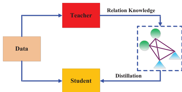
Fig. 13 A generic framework for graph-based distillation.
