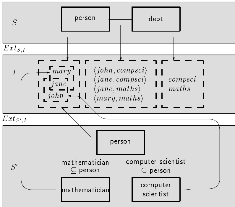
Figure 2: Two c-equivalent schemas
