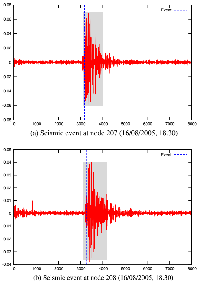
Fig. 5 Examples of non-parametric detection—the dotted vertical lines represent the top distances, the shaded areas represent the complex event
