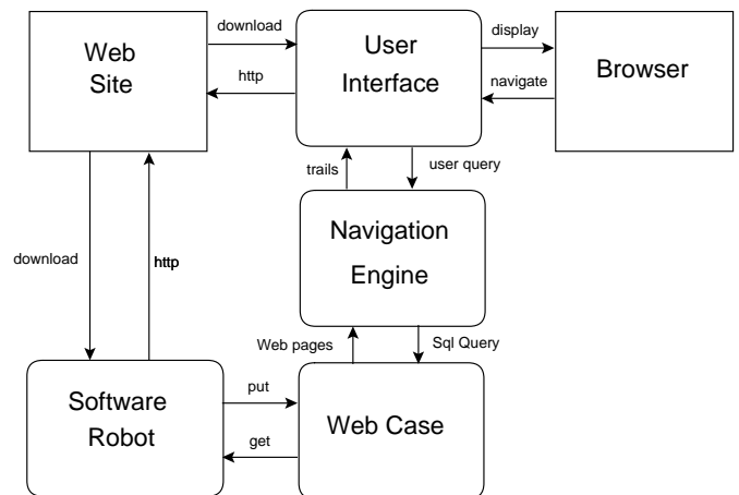
Figure 1: Navigation engine architecture
