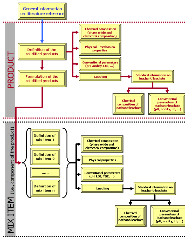
Figure 2: Schematic diagram of Monolith2's database structure, illustrated in Stegemann [2001].
