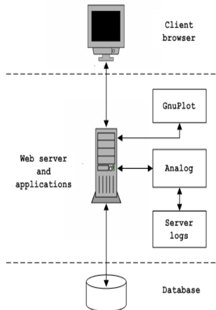
Figure 1: An abstract representation of Monolith2's architecture.
