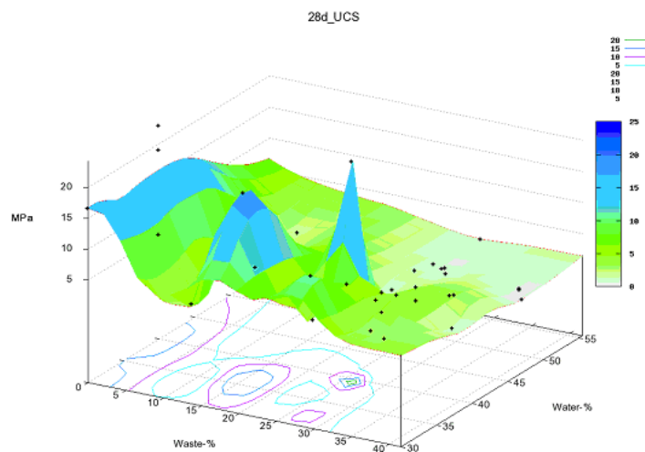
Figure 5: A plot generated by Monolith2 showing unconfined compressive strengths measured at 28 days for a variety of metal sludges treated with several different blended binder systems (the spike in strength occurs at 25% waste, 40% water and 75% binder, dry mass basis).
