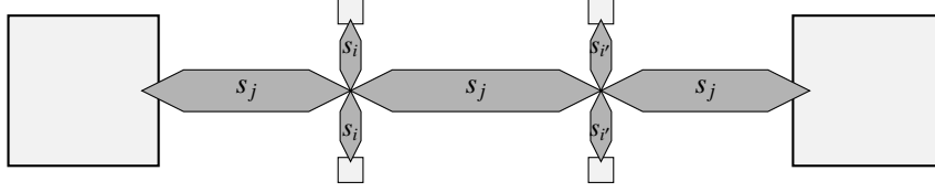
Figure 8: Encoding designs using \mathcal{RCC8c} -networks. The crossing of an edge e_j by edges e_i and e_{i'} corresponds to the ‘strings-of-sausages,’ s_j , s_i and s_{i'} , arranged as shown.
