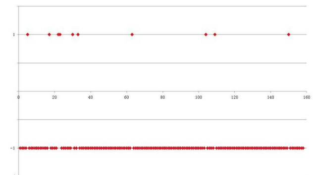
Fig. 5. Online learning with online GMMs and our online Adaboost for “httptunnel” attacks
